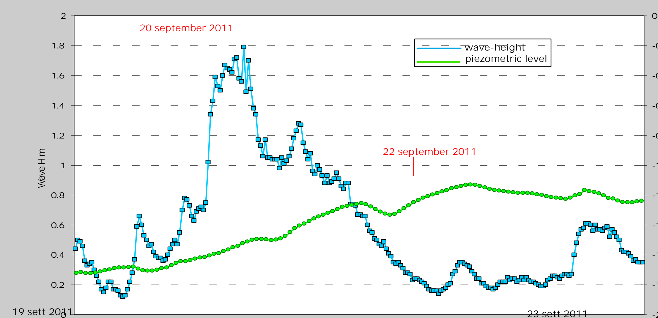
Figure 4 - Data log from the Nausicaa buoy record (wave-height) and piezometric level (from 19 to 23 September 2011)
